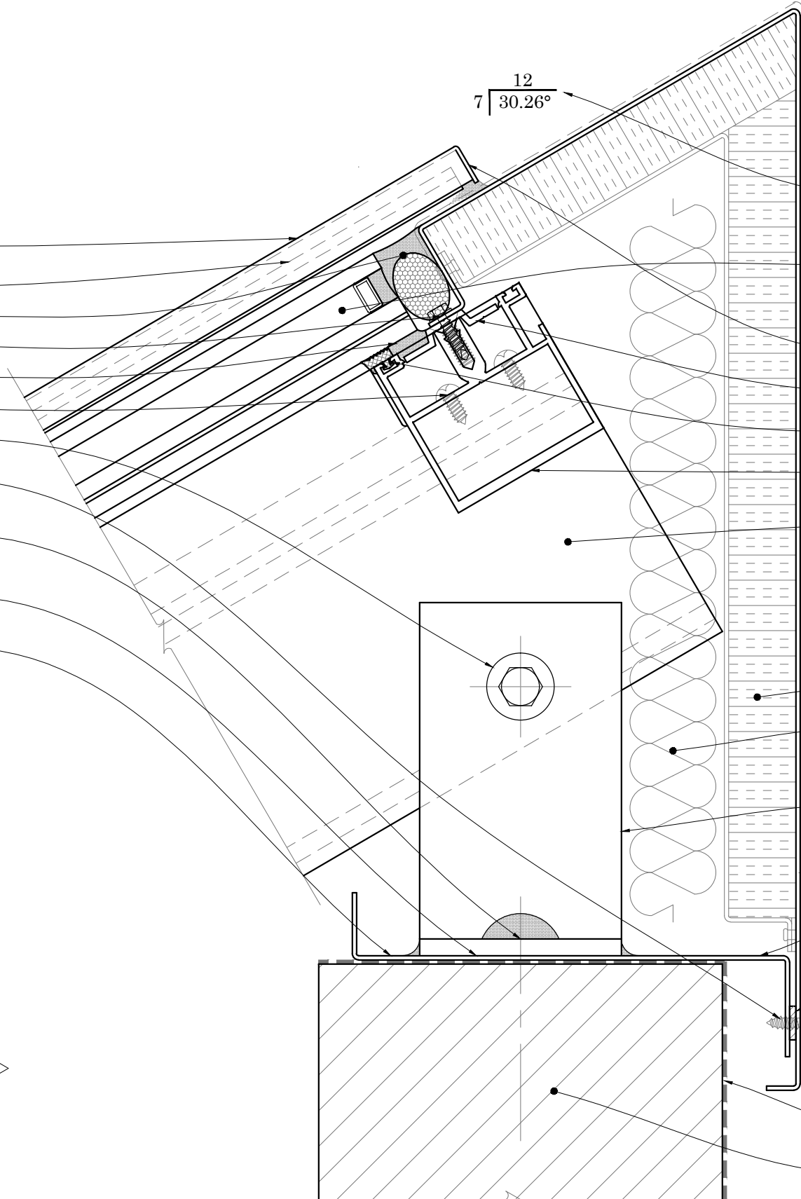
D3 RIDGE TYPICAL DETAIL
